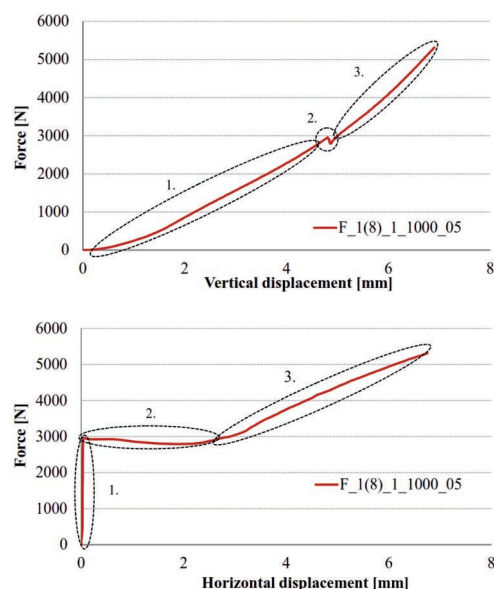
Fig. 7. a) Force vs. vertical displacement b) Force vs. horizontal displacement in the case of single float glass layer with thickness of 8 mm and height of 1000 mm; Stages of buckling behaviour of a glass column
